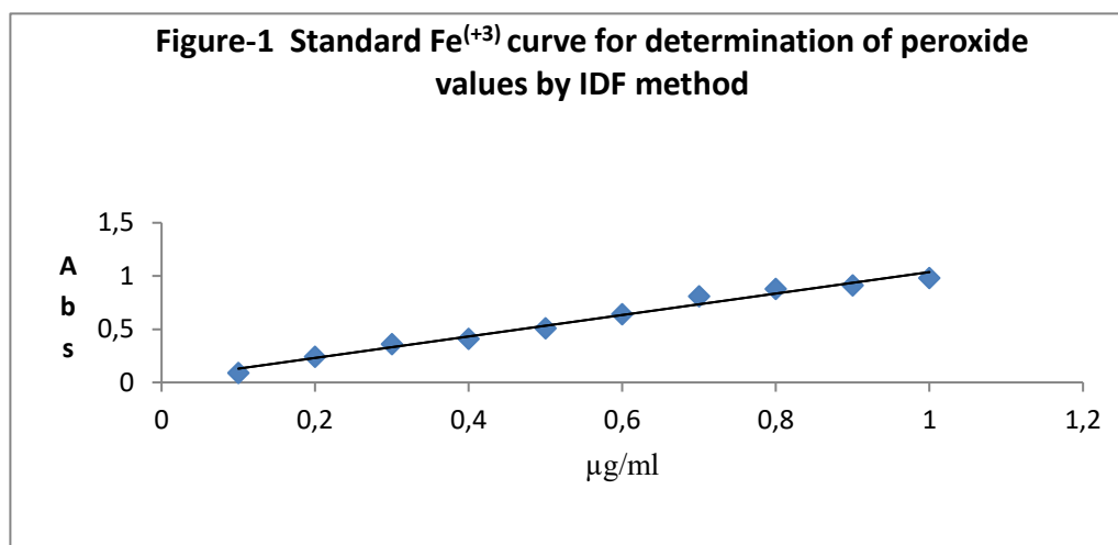
Figure. 1 Standard Fe (+3) curve for determination of peroxide values by IDF method
