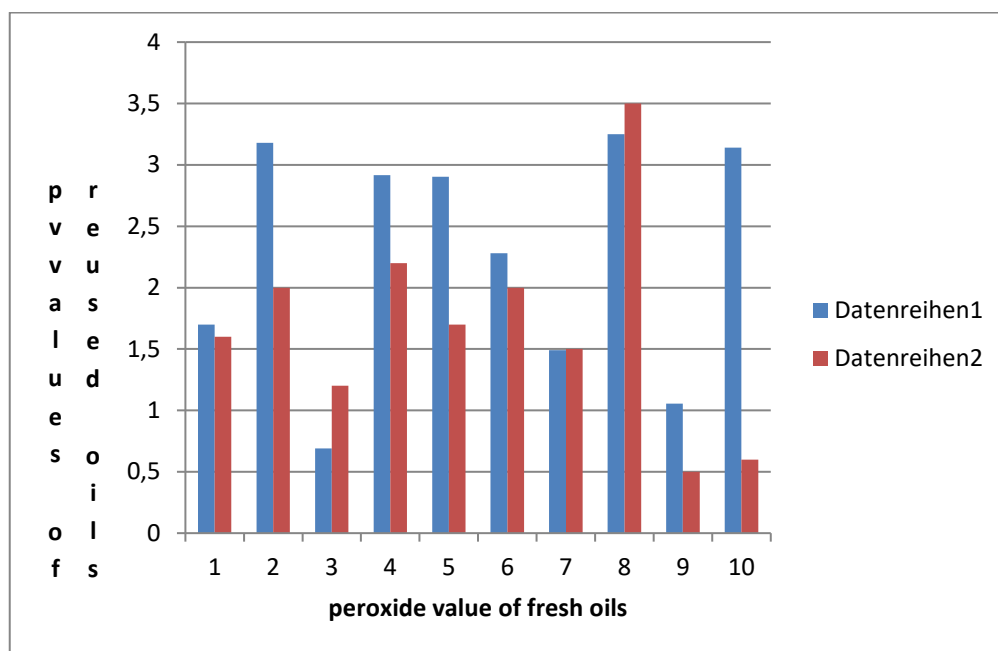
Figure.3 Plot of peroxide value of fresh oils verses peroxide values of reused oils by Iodometry method
