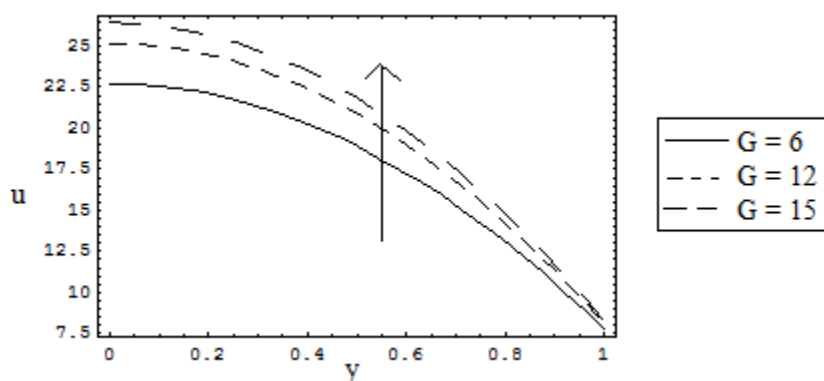
Fig. 5: Effect of G on u , when \gamma = 5, \phi = 0.1, x = 0.1, p = -25, M = 2 & \alpha = \pi/4 .
