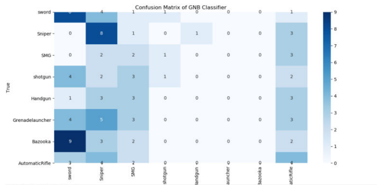
Figure 4.4: confusion matrix for GNB classifier
