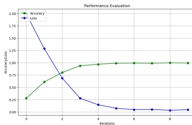
Fig 4.16 : performance evaluation of convolution neural network
