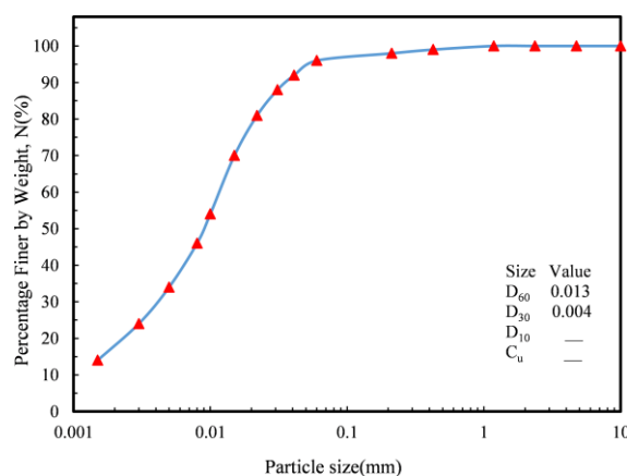
Fig. 1 Particle size distribution curve of karewa soil
