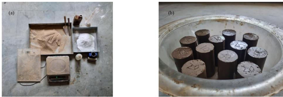
Fig. 2 (a) Sample preparation for UCS (b) UCS samples in desiccator for curing.
