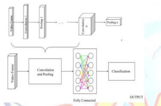
Figure2-Basic CNN Architecture
