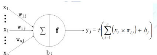
Figure 4- Activation Function [9]
