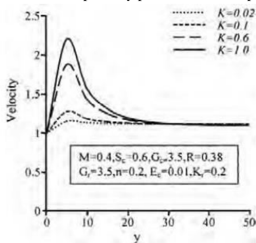
Fig. 4 – Contribution of porosity parameter on velocity field
