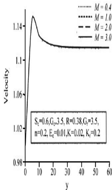
Fig.2 – Effect of magnetic parameter on velocity field
