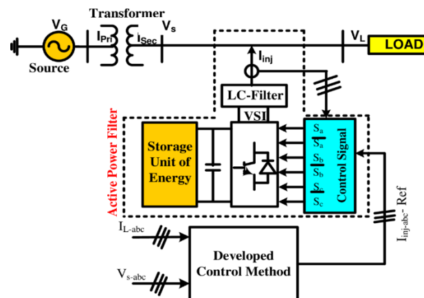
Figure 1: Controller for active power filter
