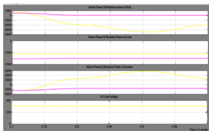
Figure 4: Simulation results: (a) PQ-Grid, (b) PQ-Load, (c) PQ-Inverter, dc-link voltage
