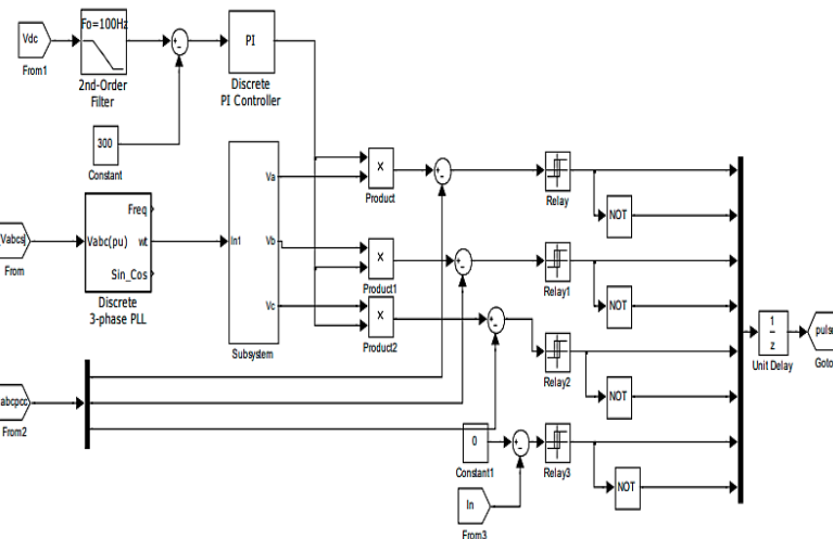
Figure 2: Simulation Diagram of Control circuit
