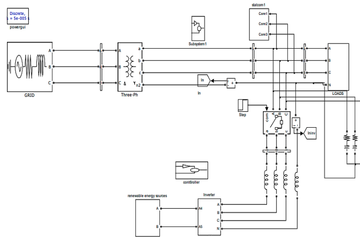
Figure 1: Simulation Diagram of proposed circuit
