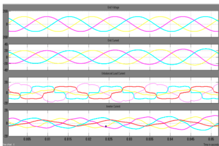
Figure 3: Simulation results: (a) Grid voltages, (b) Grid Currents Unbalanced load currents, (d) Inverter Currents
