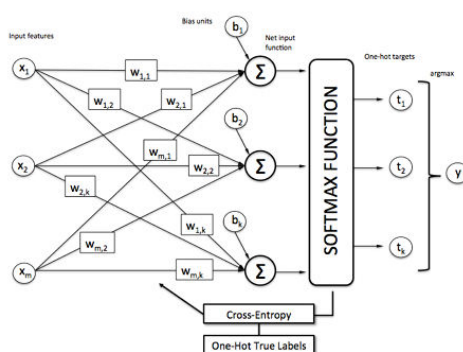
Fig. 4: Intrusion class prediction using SoftMax classifier.
