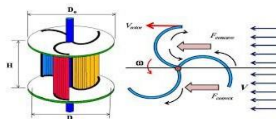
Fig.7: wind flow and rotation of turbine
