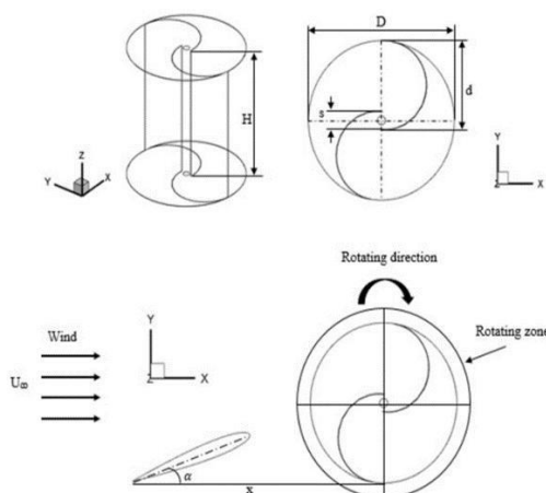
Fig.3: A sectional view of savonius wind turbine
