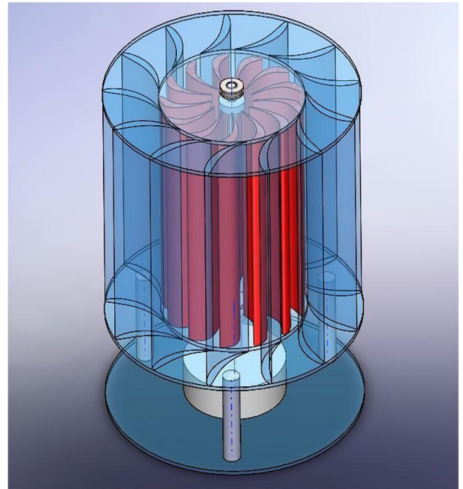
Fig.2: Savonius wind turbine
