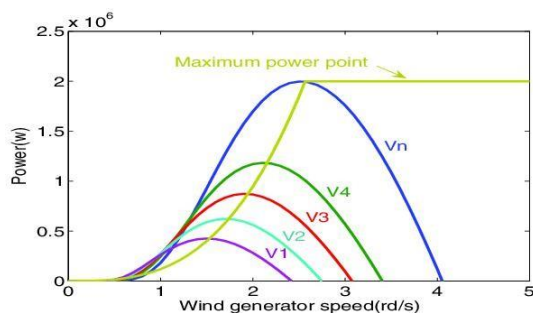
Fig.5: Characteristics of PMSG
