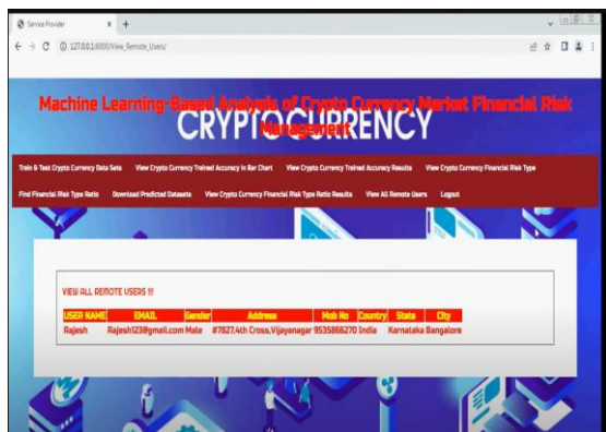
Fig.1. Home page.
