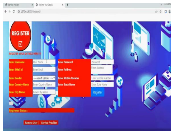
Fig.2. user login
