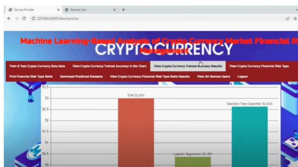
Fig.6. graph analysis.
