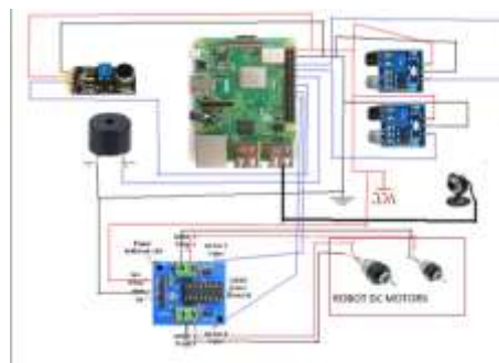
Figure 7: circuit diagram
