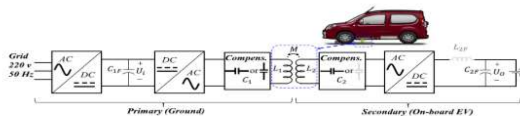
Figure.4. General Block diagram for a contactless charger for EV.
