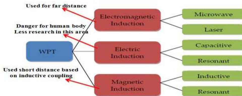
Figure. 2 Different Types of WPT
