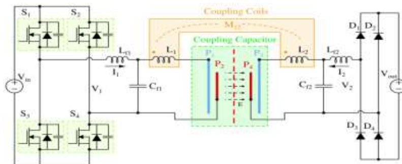
Figure.5. Circuit Topology of the LC compensated IPT-CPT System.
