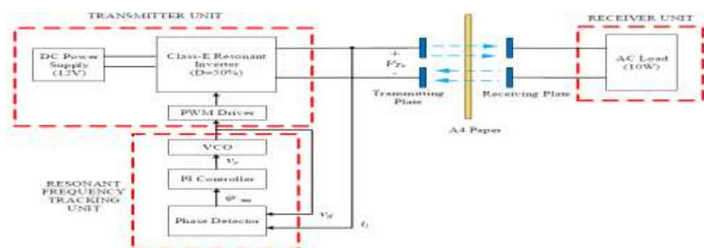
Figure.3. Proposed CPT System with FTU Block Diagram.
