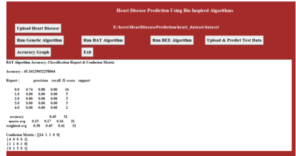
Fig.4. BAT Accuracy.
