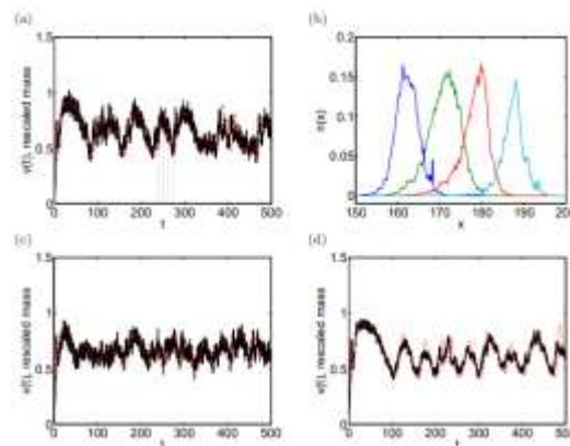
Fig. 7 Oscillations in the wave speed of the hybrid model (2.2)–(2.6) and (2.10). (a) Wave speed in comparison to current number of particles for N_0 = 10,000 , \tau_a = 4 . Solid line: wave speed, dashed line: number of particles, dotted lines: times of wave forms shown in panel (b). (b) Waveform at 4 distinct times marked in panel (a) from left to right. (c) As in (a) with N_0 = 10,000 , \tau_a = 2 . (d) As in (a) with N_0 = 50,000 , \tau_a = 4 . Other parameters are given in Section 5.3.
