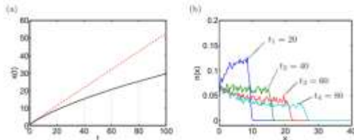
80 Fig. 2 Numerical solutions of the hybrid chemotaxis model (2.2)–(2.6) and (2.10) without growth and death terms. (a) Comparison of position of wave front over time. Solid line: without growth/death ( \alpha = 0 ), dashed line: with growth/death ( \alpha = 1 ). (b) Wave form at different times during simulation with \alpha = 0 . From left to right: t = 20, 40, 60, 80 . Remaining parameters as in Figure2.
