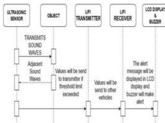
Fig 4. Sequence diagram of distance calculation
