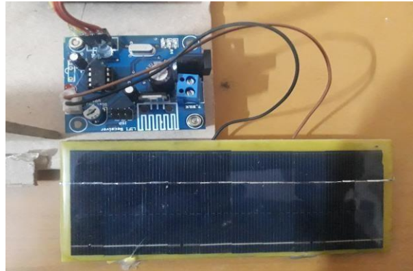
Fig 8. Li-Fi Receiver
