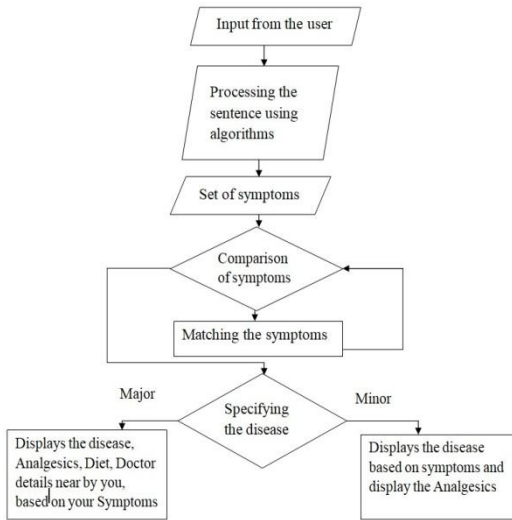
Figure 3: Data Flow Diagram
