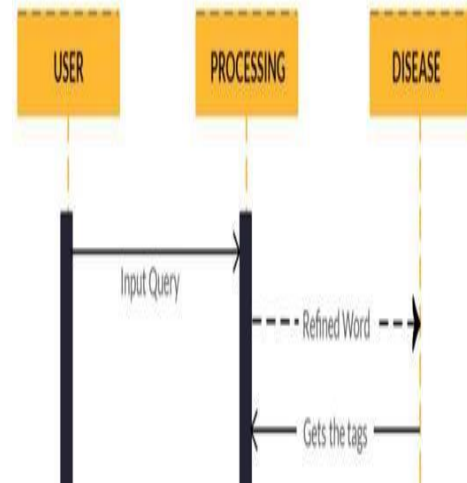
Figure 5 Sequence Diagram
