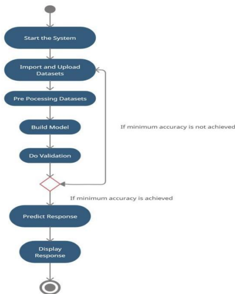
Figure 8 State/Activity Diagram
