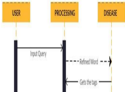
Figure 7 Interaction Diagram
