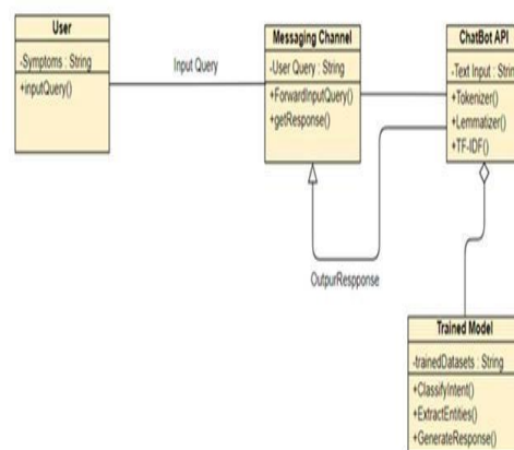
Figure 6 Class Diagram
