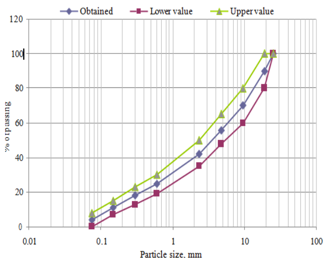
Graph:3.3. Grain size distribution of aggregate gradation
