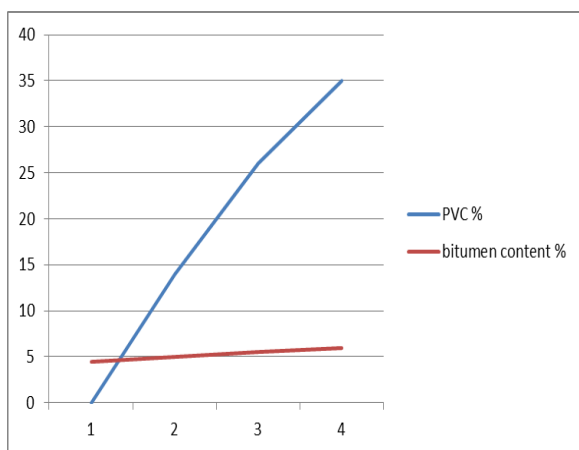
Graph:4.4.Variation of PVC value with bitumen content at different coal ash content
