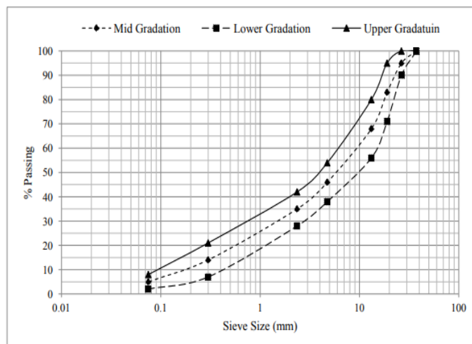
Graph:3.2. Aggregate Gradation of Dense Bituminous Macadam (DBM) Mix
