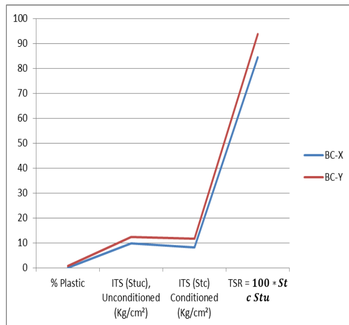
Graph:4.3. Indirect tensile strength (ITS) and TSR variations
