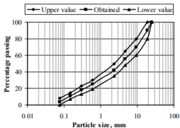
Figure: 3.5..Grain size distribution of aggregate gradation
