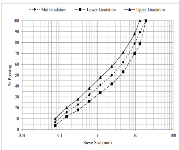
Graph:3.1. Aggregate Gradation of Bituminous Concrete (BC) mix
