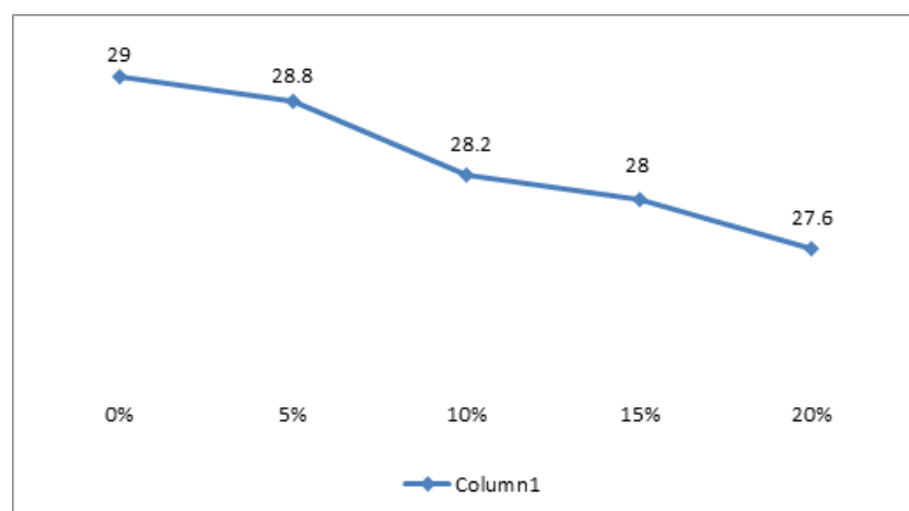
Graph: 3.1: Slump cone test
