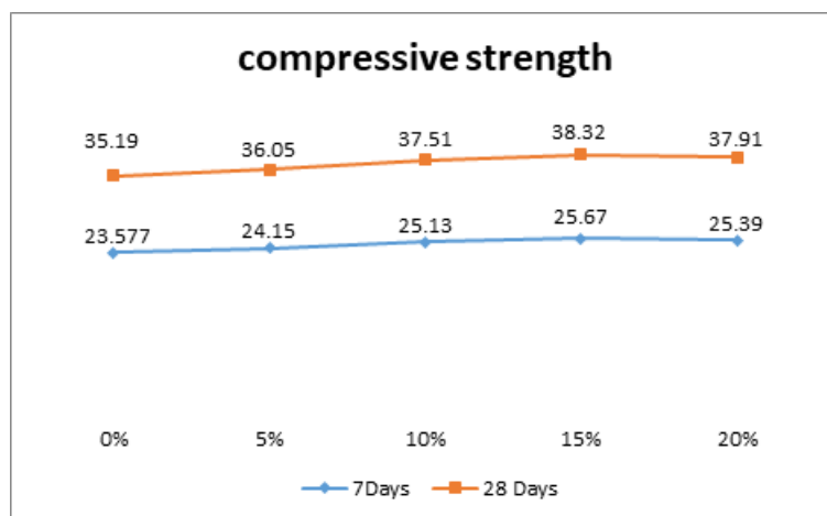
Graph: 3.2: Compressive strength of M30 concrete with varying % of Metakaolin
