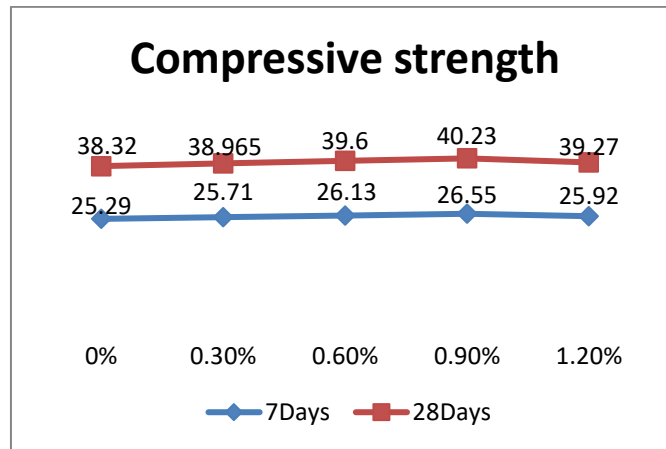
Graph: 3.3: Compressive strength of M30 concrete with optimum % of metakaolin and varying the % of polypropylene fiber
