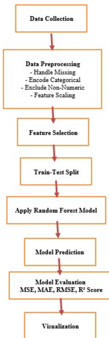
Fig 1. Methodology Flowchart
