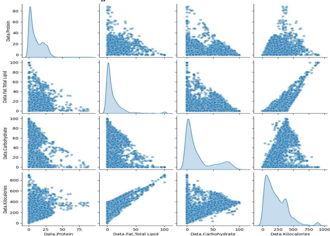
Fig 3. The relationships between different variables
