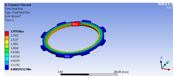
Figure 20 heat flux in grey cast iron
