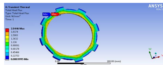
Figure 24 heat flux in ZAMAK
