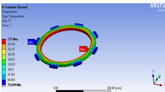
Figure 19 temperature distributions in AL7075
