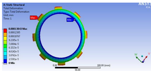
Figure 17 total deformation in ZAMAK
