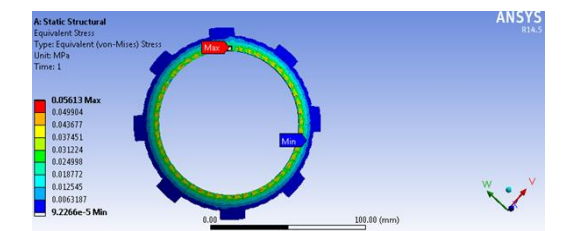
Figure 16 stress in ZAMAK
