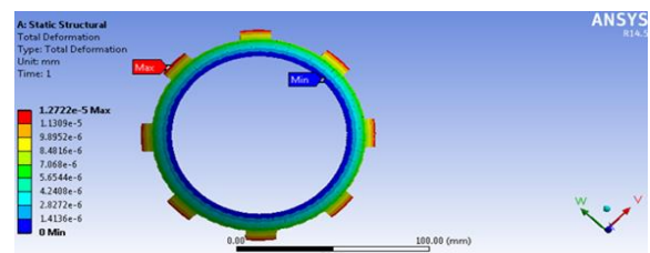
Figure 15 total deformation in SF001
