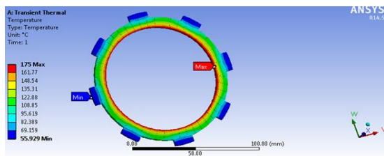
Figure 25 temperature distributions IN ZAMAK
