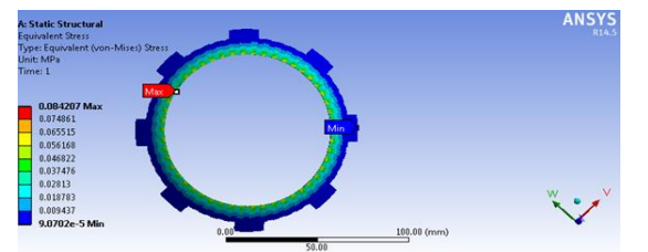
Figure 14 stress in SF001
