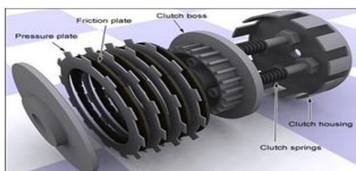
Figure 1 multi clutch nomenclature
