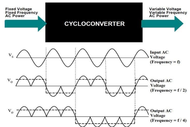
Fig.16 CYCLOCONVERTER WAVEFORMS
