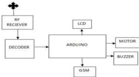
Fig 2. Helmet Circuitry
