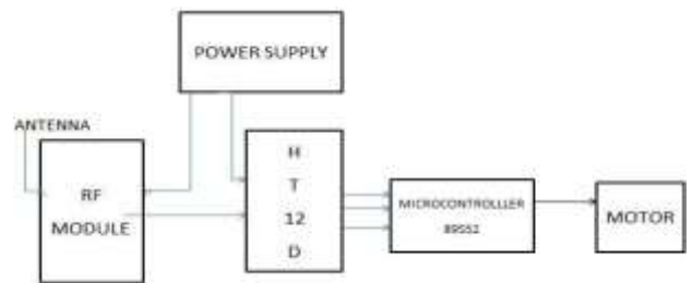
Fig 5 Block Diagram for Bike Unit
