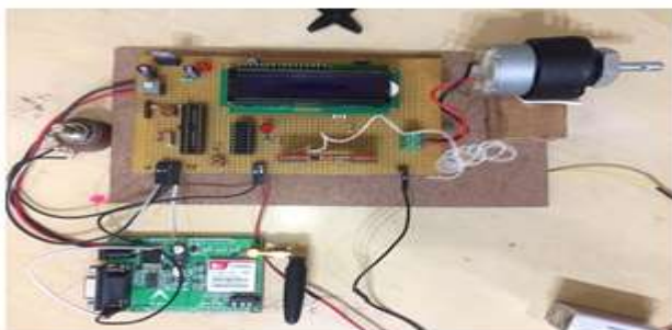
Fig 4. Helmet Circuitry 2
