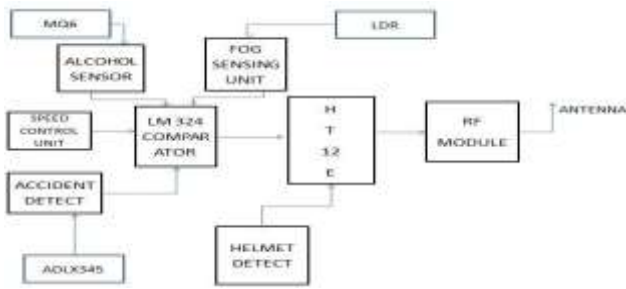
Fig 1. Block Diagram for Helmet Unit
