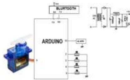
Fig:8. circuit Diagram
