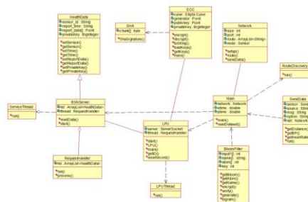
Fig 2: Class diagram
