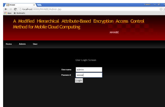
Fig.6: Admin Screen
