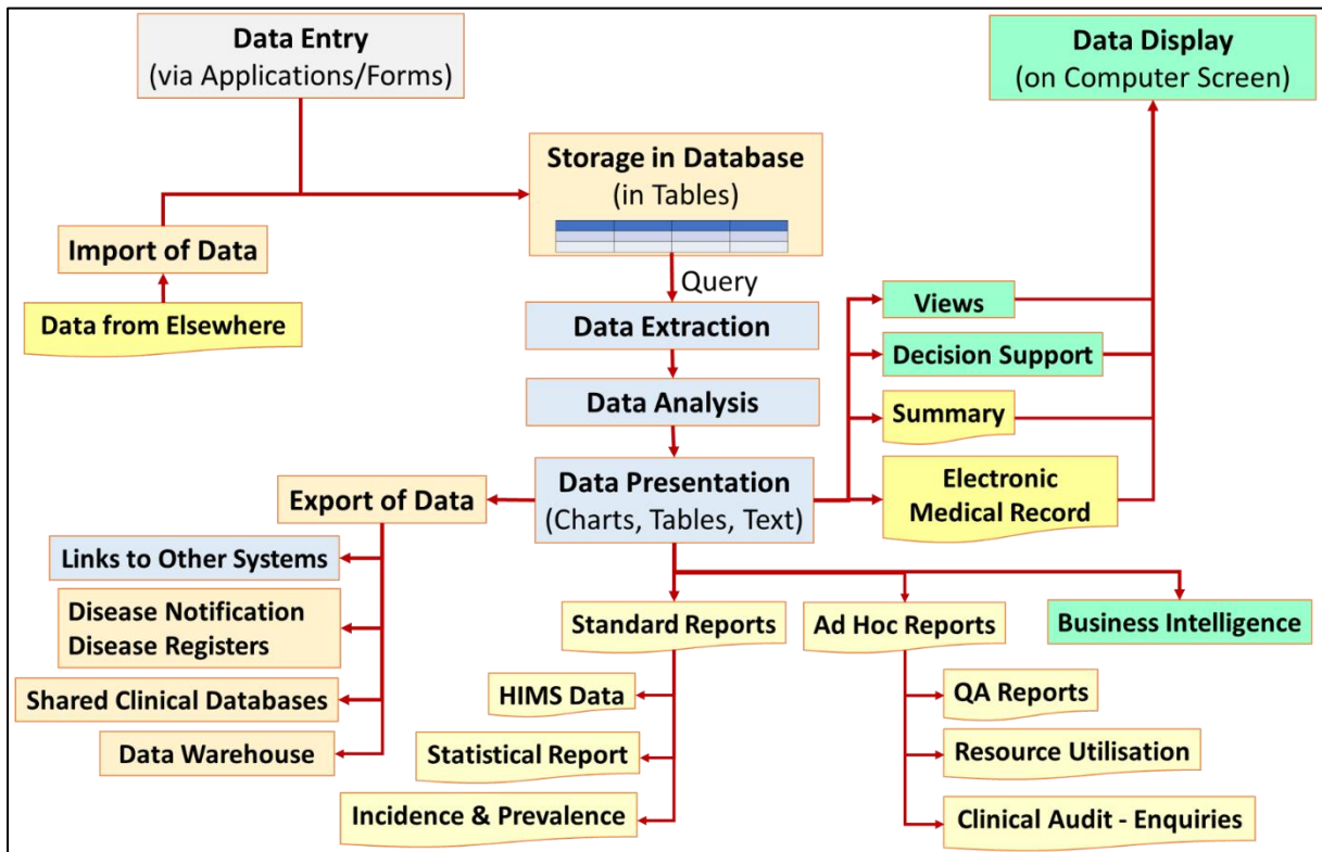
Fig 3.2 System Design
