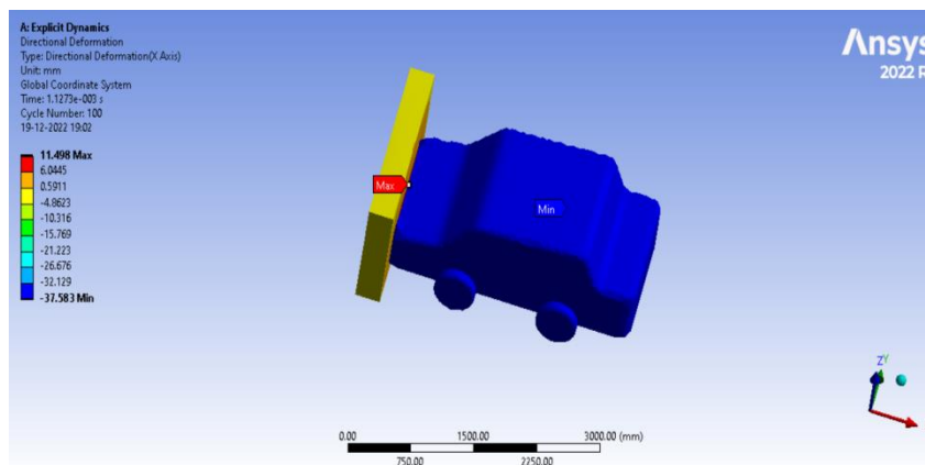
Figure 20: Directional deformation
