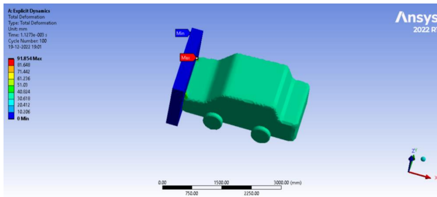
Figure 19: Total deformation
