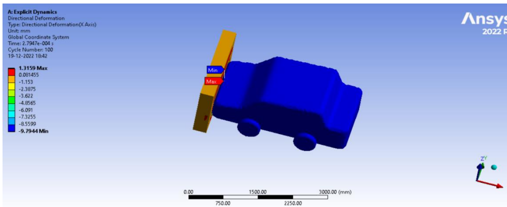
Figure 16: Directional deformation
