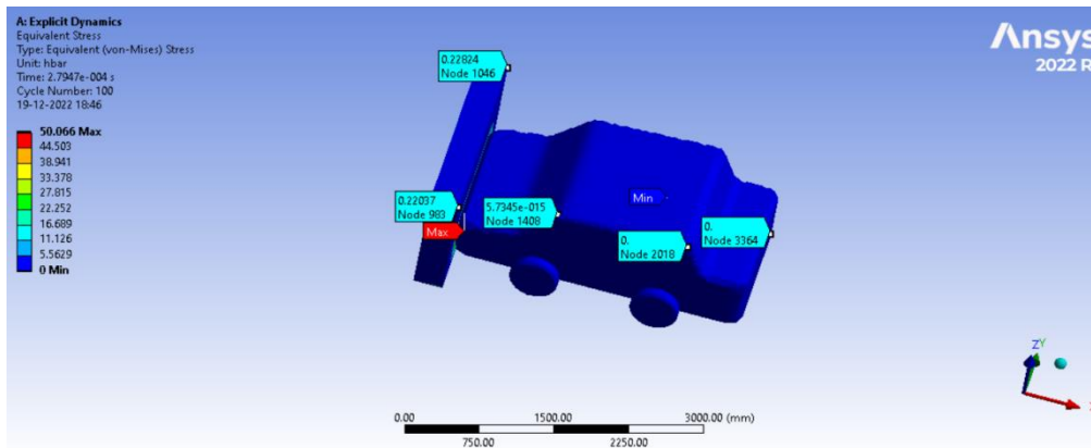
Figure 17: Equivalent stress
