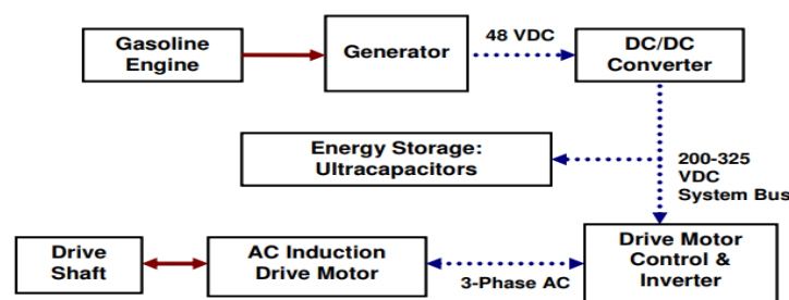
Figure 1: Block Diagram of our Series Hybrid System
