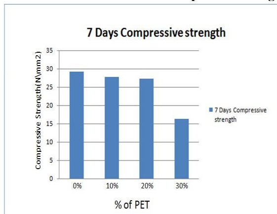
Graph: 7 days compressive strength
