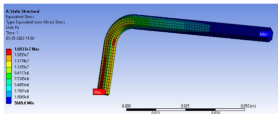
Figure 9 equivalent stresses of stainless steel round bar
