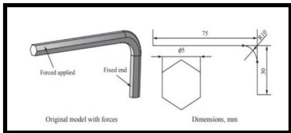
Figure 4 dimensions of hexaallen key
