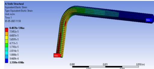
Figure 11 equivalent strain of stainless steel round bar
