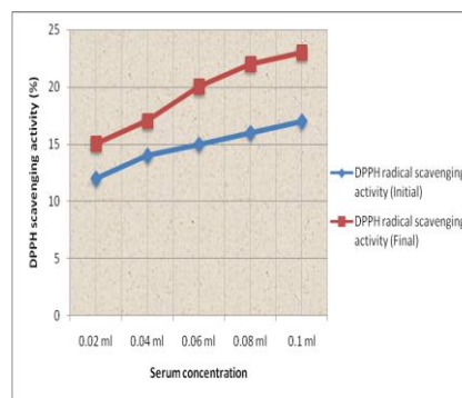
Fig. 3 DPPH radical scavenging activity of subject C (before and after supplementation)
