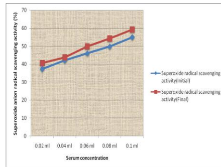
Fig. 14 Superoxide anion radical scavenging activity of subject D (before and after supplementation)
