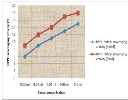
Fig. 4 DPPH radical scavenging activity of subject D (before and after supplementation)
