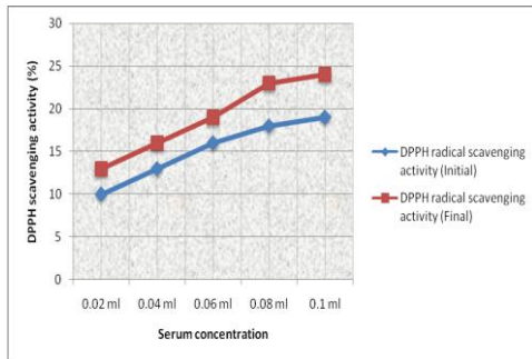
Fig. 5 DPPH radical scavenging activity of subject E (before and after supplementation)
