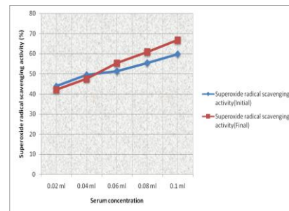
Fig. 15 Superoxide anion radical scavenging activity of subject E (before and after supplementation)
