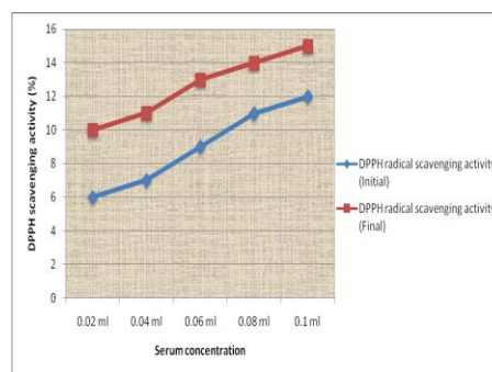
Fig. 1 DPPH radical scavenging activity of subject A (before and after supplementation)
