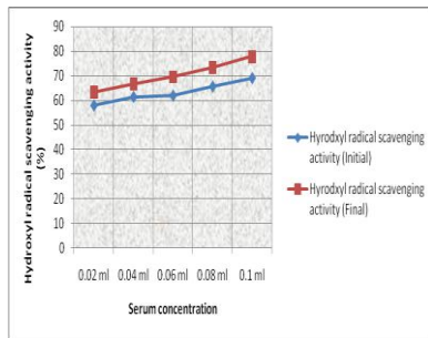
Fig. 10 Hydroxyl radical scavenging activity of subject E (before and after supplementation)
