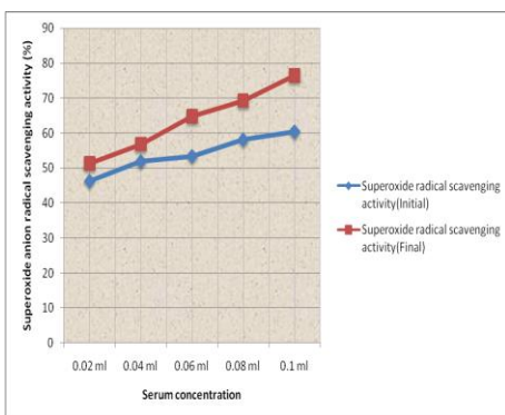
Fig.13 Superoxide anion radical scavenging activity of subject C (before and after supplementation)
