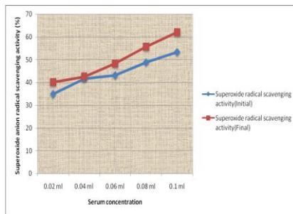
Fig.11 Superoxide anion radical scavenging activity of subject A (before and after supplementation)
