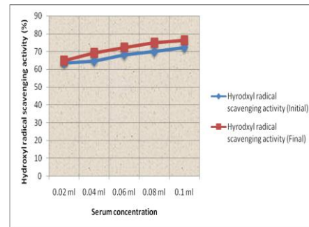
Fig. 8 Hydroxyl radical scavenging activity of subject C (before and after supplementation)
