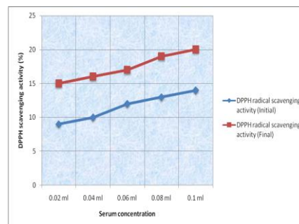
Fig. 2 DPPH radical scavenging activity of subject B (before and after supplementation)
