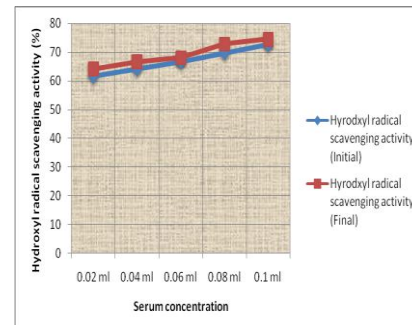
Fig. 9 Hydroxyl radical scavenging activity of subject D (before and after supplementation)
