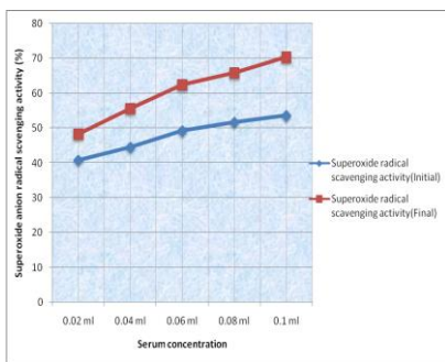
Fig. 12 Superoxide anion radical scavenging activity of subject B (before and after supplementation)
