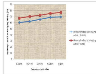
Fig.6 Hydroxyl radical scavenging activity of subject A (before and after supplementation)
