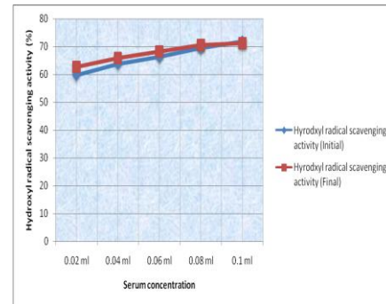
Fig. 7 Hydroxyl radical scavenging activity of subject B (before and after supplementation)
