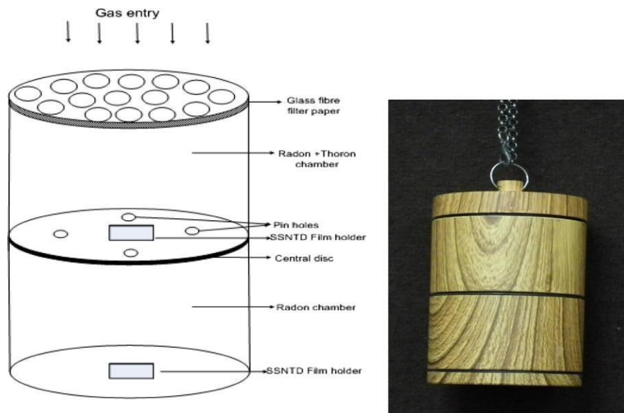
Fig. 1 schematic diagram of pin hole dosimeter.
