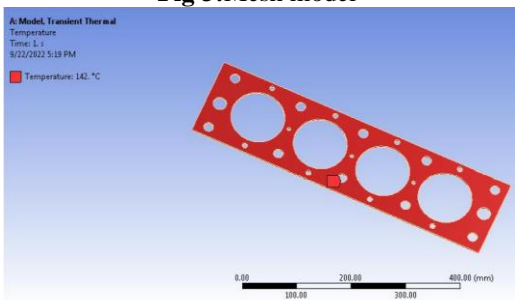
Fig 4: Temperature
