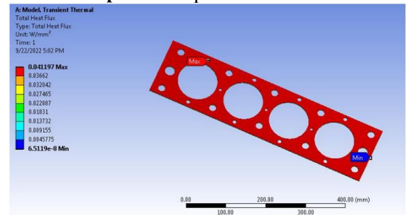
Fig 20: Total Heat Flux
