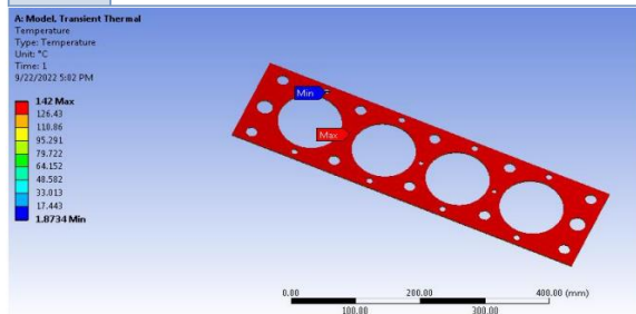
Fig 19: Temperature
