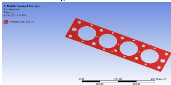
Fig 24: Temperature
