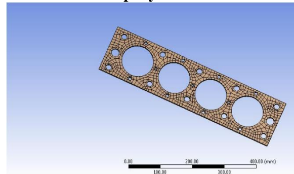
Fig 16: Mesh
