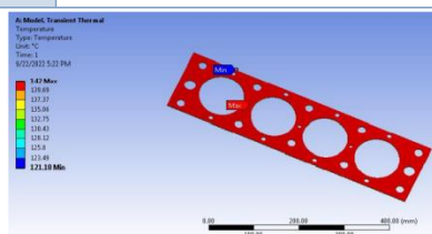
Fig 5: Temperature
