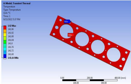
Fig 12: Temperature
