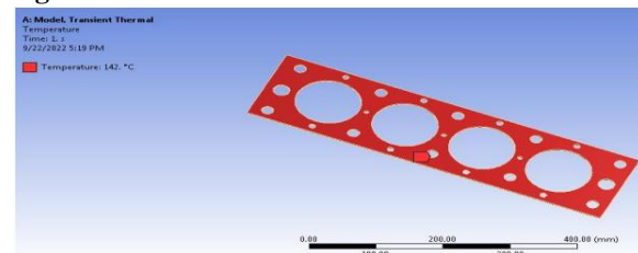
Fig 17: Temperature
