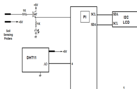
Fig 8. Schematic Diagram
