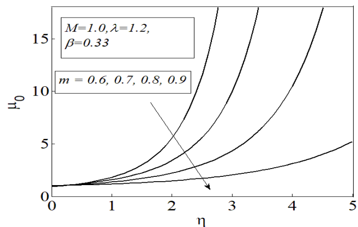
Fig.4. Variation of velocity profiles \mu_0 with \eta for m = 0.6, 0.7, 0.8, 0.9 , \lambda = 1.2 , \beta = 0.33 and M = 1.0 .
