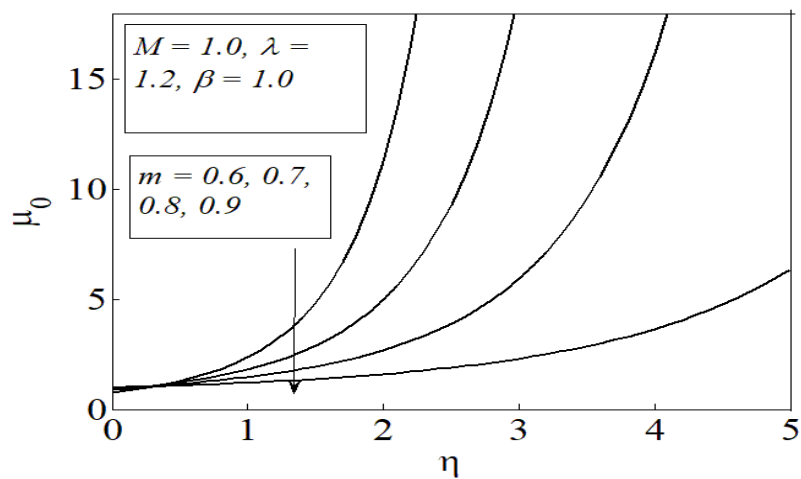
Fig.5. Variation of velocity profiles \mu_0 with \eta for m = 0.6, 0.7, 0.8, 0.9 , \lambda = 1.2 , \beta = 1.0 and M = 1.0 .
