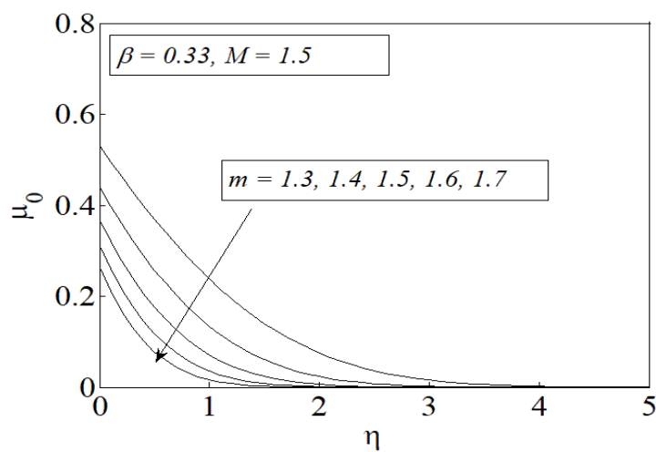
Fig.7. Variation of velocity profiles \mu_0 with \eta for m = 1.3, 1.4, 1.5, 1.6, 1.7 , \beta = 0.33 and M = 1.5 .
