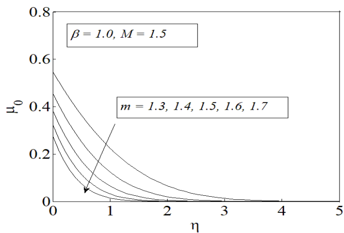
Fig.6. Variation of velocity profiles \mu_0 with \eta for m = 1.3, 1.4, 1.5, 1.6, 1.7 , \beta = 1.0 and M = 1.5 .
