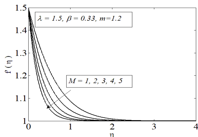
Fig.2. Variation of velocity profiles f'(\eta) with \eta for M=1,2,3,4,5 , \lambda=1.5 , \beta=0.33 and m=1.2 .
