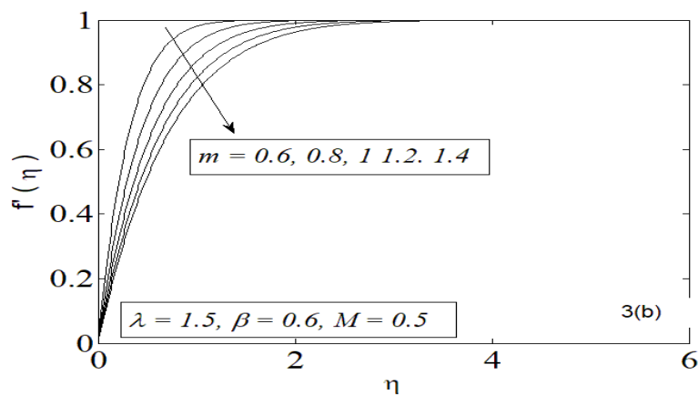
Fig.3(b). Variation of velocity profiles f'(\eta) with \eta for m = 0.6, 0.8, 1.0, 1.2, 1.4 , \lambda = 1.5 , \beta = 0.6 and M = 0.5 .
