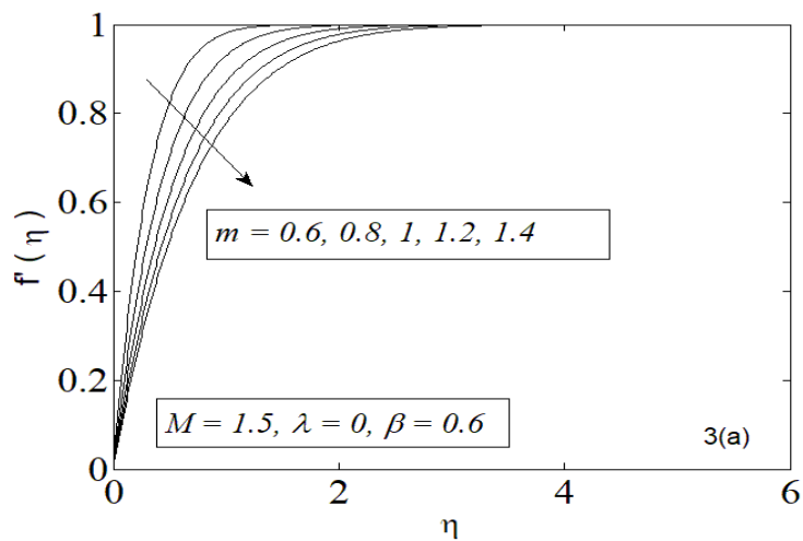
Fig.3(a). Variation of velocity profiles f'(\eta) with \eta for m = 0.6, 0.8, 1.0, 1.2, 1.4 , \lambda = 0 , \beta = 0.6 and M = 1.5 .
