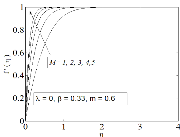
Fig. 1. Variation of velocity profiles f'(\eta) with \eta for M=1,2,3,4,5 , \lambda=0 , \beta=0.33 and m=0.6
