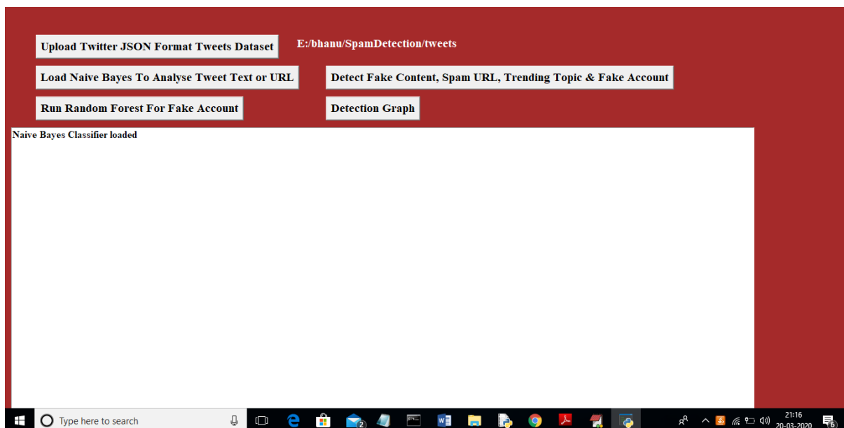
Fig 4.4 In above screen naïve bayes classifier loaded and now click on ‘Detect Fake Content, Spam URL, Trending Topic & Fake Account’ to analyse each tweet for fake content, spam URL and fake account using Naïve Bayes classifier and other above mention technique
