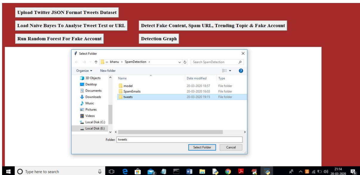
Fig 4.2 In above screen I am uploading ‘tweets’ folder which contains tweets from various users in JSON format. Now click open button to start reading tweets
