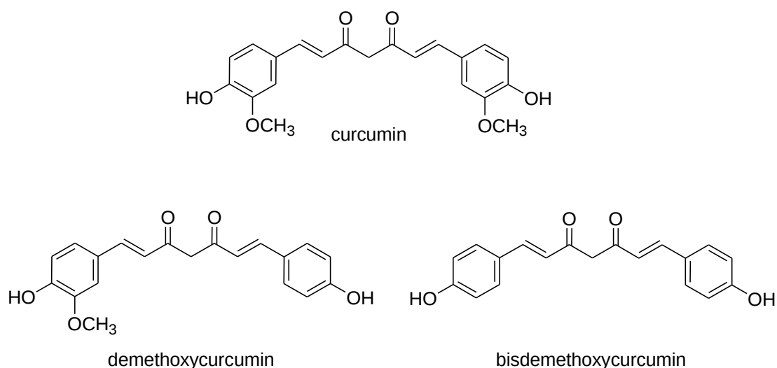
Figure 1 : Structure of the 3 major curcuminoids in turmeric
