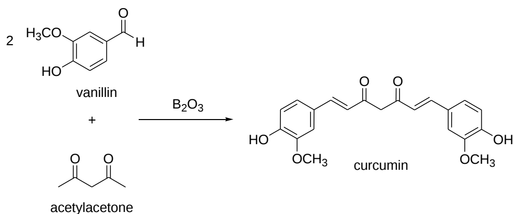
Scheme 2: Synthesis of curcumin according to Pavolini 33
